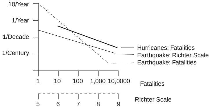
EXHIBIT 9.4 Power-Law Distributions of Hurricane and Earthquake Frequency and Severity
