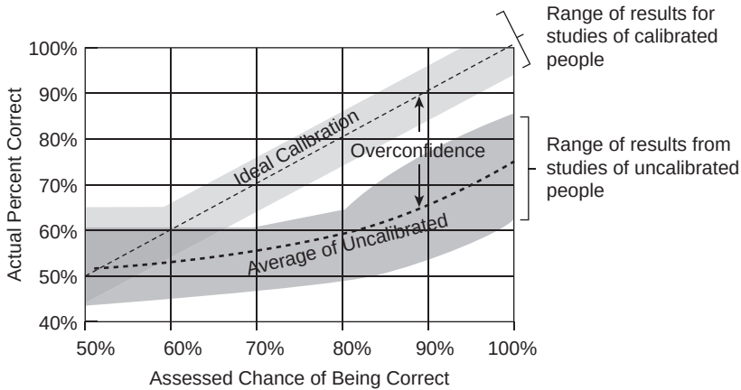
EXHIBIT 6.2 Comparison of Uncalibrated and Calibrated Individuals
