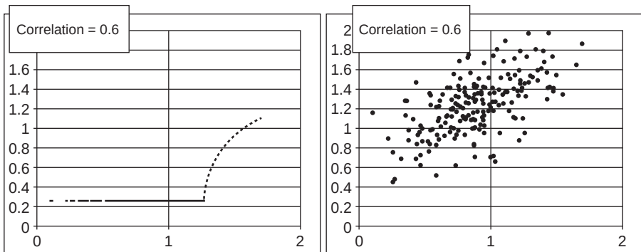
EXHIBIT 9.7 Same Correlation Coefficient, Very Different Patterns
