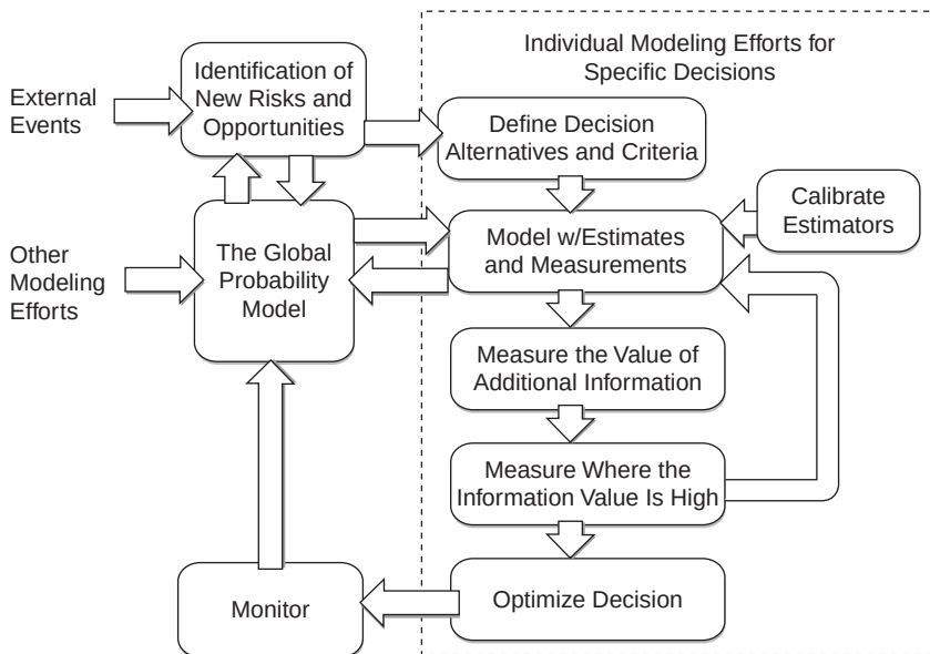
EXHIBIT 12.1 Evolving Global Probability Model
