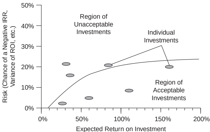
EXHIBIT 7.6 Risk versus Return: The Investment Boundary
