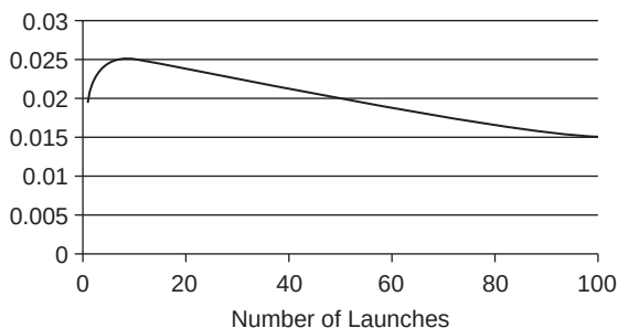
EXHIBIT 11.2 Conditional Robust Bayesian Method: Chance of Shuttle Disaster after Each Observed Near Miss (e.g., Falling Foam, O-Rings Burning Through) with an Otherwise Successful Launch
