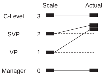
Relative Impact of IT Project Failure Rates Using a 0-to-3-Point Scale for “IT Project Sponsor” vs. Actual Historical Impact
