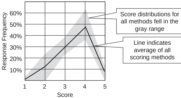
EXHIBIT 7.4 Distribution of Scores from Seven Different 5-Point Scales
