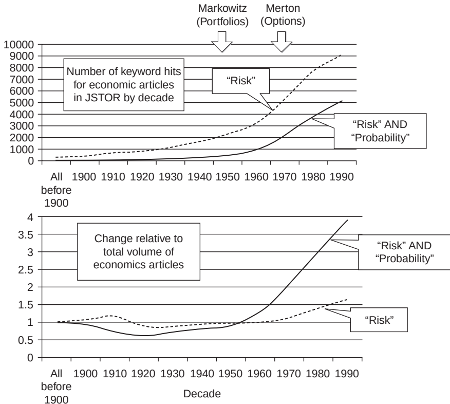
EXHIBIT 4.1 Risk and Probability in Economic Literature
