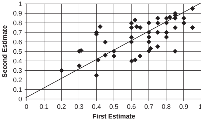
EXHIBIT 6.4 Agreement between First and Second Estimates of IT Project Failure Probabilities
