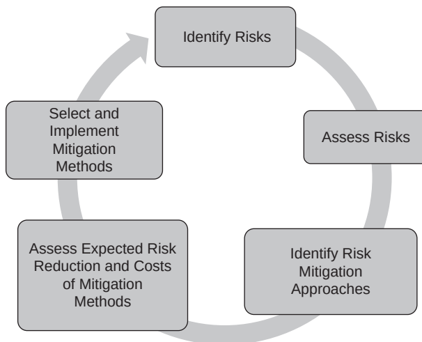
EXHIBIT 2.2 A (Simplified) Risk Management Cycle
