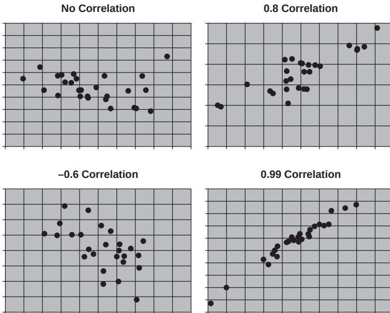
EXHIBIT 9.6 Examples of Correlated Data
