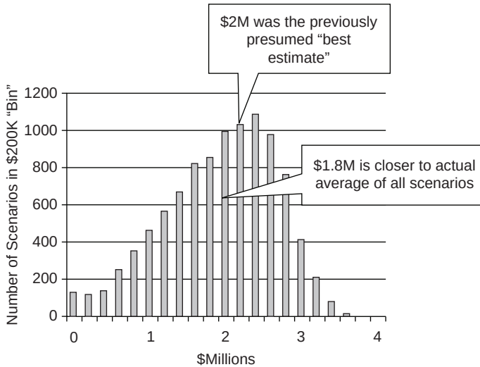
EXHIBIT 9.1 Histogram of Outcomes
