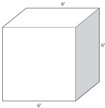
Figure 1.2 Cube
