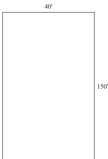
Figure 1.1 Rectangle
