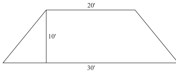
Figure 1.5 Trapezoid
