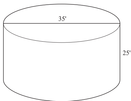
Figure 1.4 Cylinder
