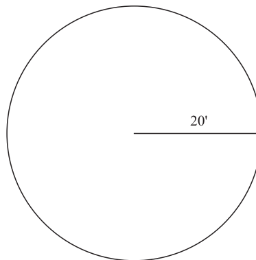
Figure 1.3 Circle
