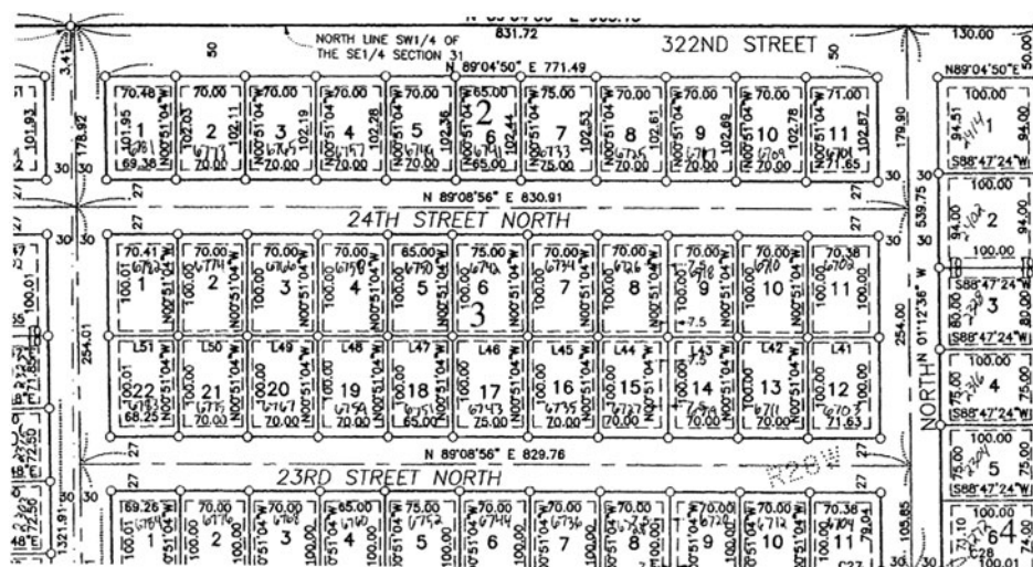
Figure 4.8 Plat drawing
