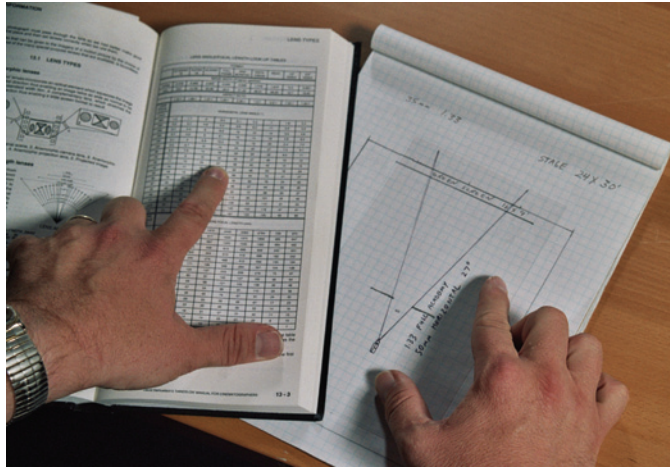
Figure 9.12: Lens angles drawn on clear acetate sheets are a quick way to plan out camera position on graph paper. Each square represents 1 square foot. The small box in front of the camera represents the candy bar. By counting the squares it can be seen that the candy is 15 feet away from the screen. Lens angles for any focal length and format can be found by consulting camera manuals or making use of lens calculators. This table is shown in Figure 9.14.
