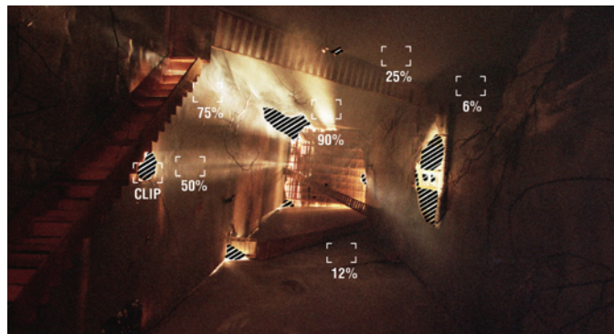
Figure 10.25: With a digital video camera, areas above 90 percent are clipped and show no more gradations. These areas are represented by the zebra pattern over “blown out” portions of the image. The other readings are percentages of brightness as seen through the viewfinder of the camera. Note that the 50 percent reading coincides with the zone 5 middle gray of the photographic process.
