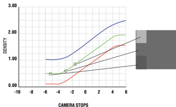
Figure 5.10: An underexposed gray card.
