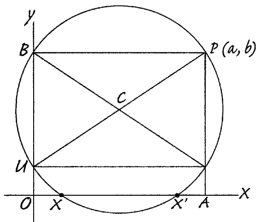
FIG. 6. GRAPHICAL SOLUTION OF A QUADRATIC EQUATION WITH REAL ROOTS
