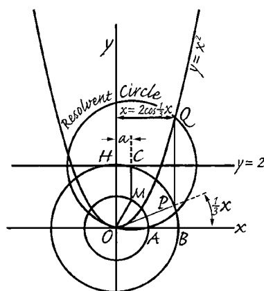
FIG. 5. PARABOLA AS AN ANGULAR TRISECTOR
