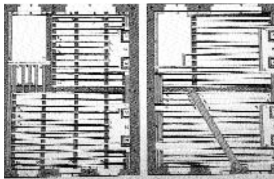
Figure 14.20 Timber floor construction from Peter Nicholson, The New and Improved Practical Builder and Workman's Companion , 1823
