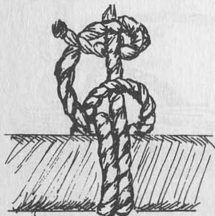
FISHERMAN'S BEND
