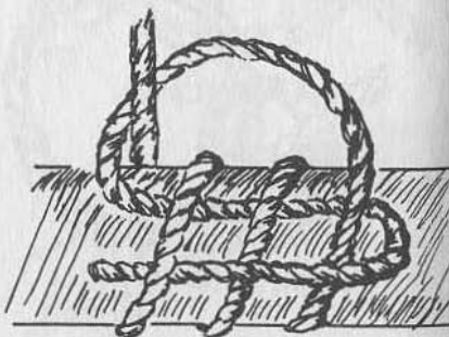
HALYARD BEND
