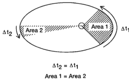
Figure 2-3. Area/time relationship. Kepler's second law reveals that the velocity of an object changes with orbital radius.
