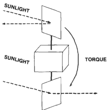
Figure 8-6. Solar radiation propeller torque.
