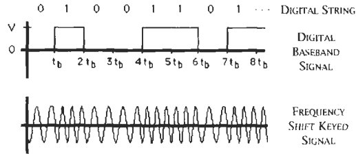
Figure 5-13. Frequency shift keying modulation. The change in frequency of the carrier wave is used to represent the digital baseband signal.
