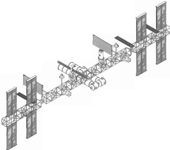
Figure 1-16. International space station. This 1993 concept shows the basic building blocks of the planned space station: habitation and laboratory modules supported by solar power arrays and other systems on a long truss structure.
