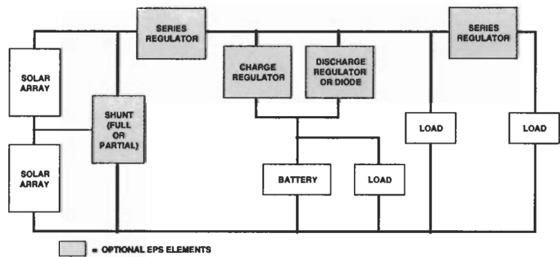
Figure 8-9. Electrical power subsystem configuration options.
