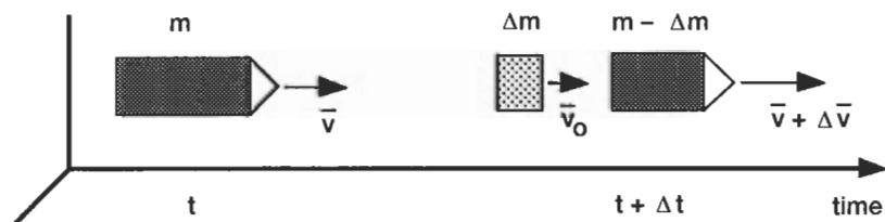
Figure 3-1. Rocket momentum. A rocket trades momentum with its exhausted propellant to produce thrust and increase velocity.
