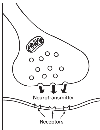
Chemical synapse
