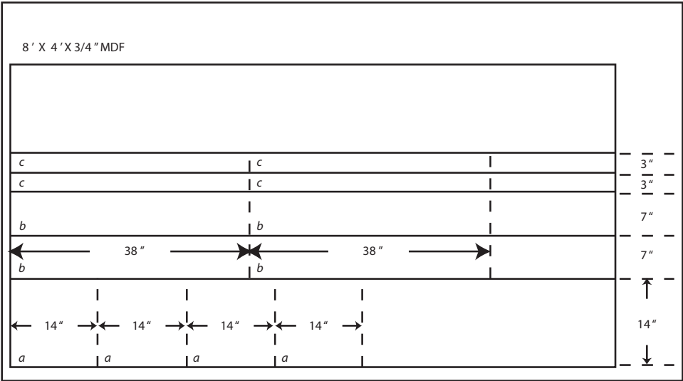
FIGURE 12.6 Speaker stand cutout list
