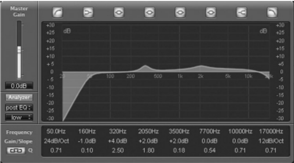
FIGURE 10.6 Multiband EQ
