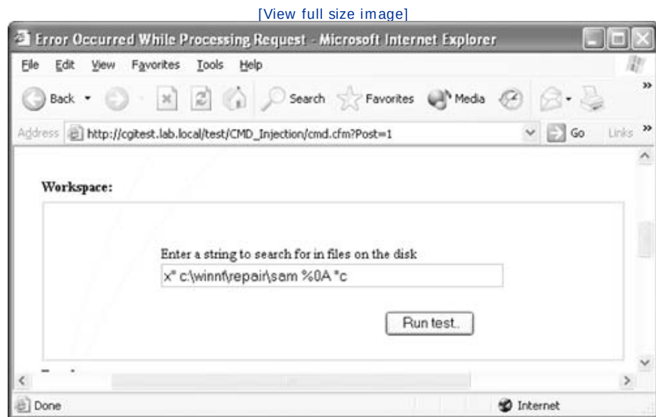
Figure 4-4. The example code renders an input window that looks like a search form. An attacker can exploit the code using well-crafted input. Some clever escaping is shown. Note in particular the " character.
