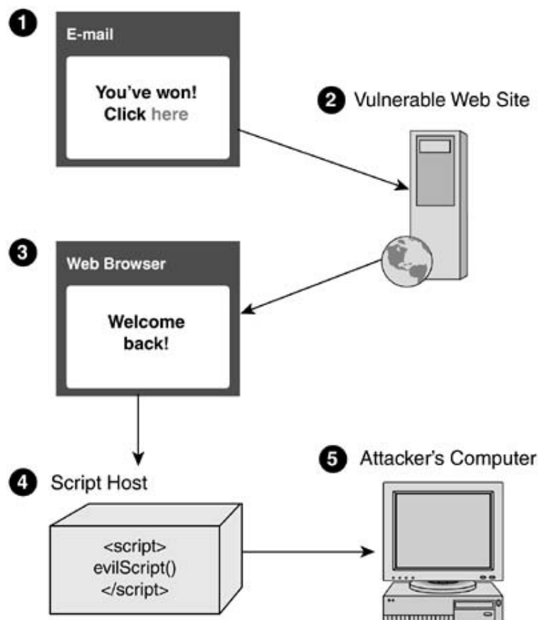
Figure 5-1. XSS illustrated. The attacker sends active content to a vic which invokes a script on the vulnerable Web site (2). Later, once inv Web browser, hitting the vulnerable Web site (3), the script runs (· allows the attacker access (5).
