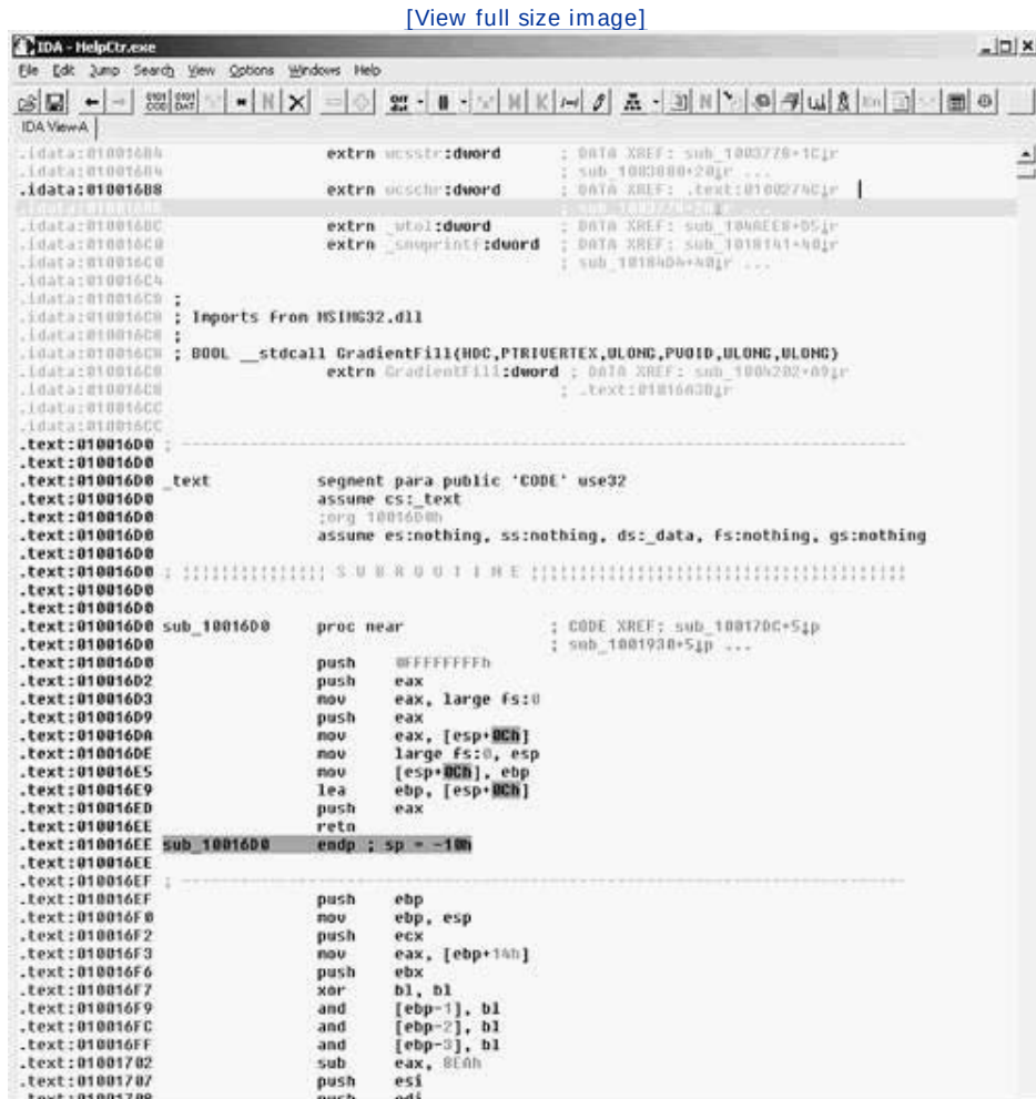
Figure 3-4. A screen shot of IDA-Pro reverse assembling the program helpctr.exe , which is included as part of the Microsoft Windows XP OS. In this exercise, we explore helpctr.exe for a buffer overflow vulnerability.
