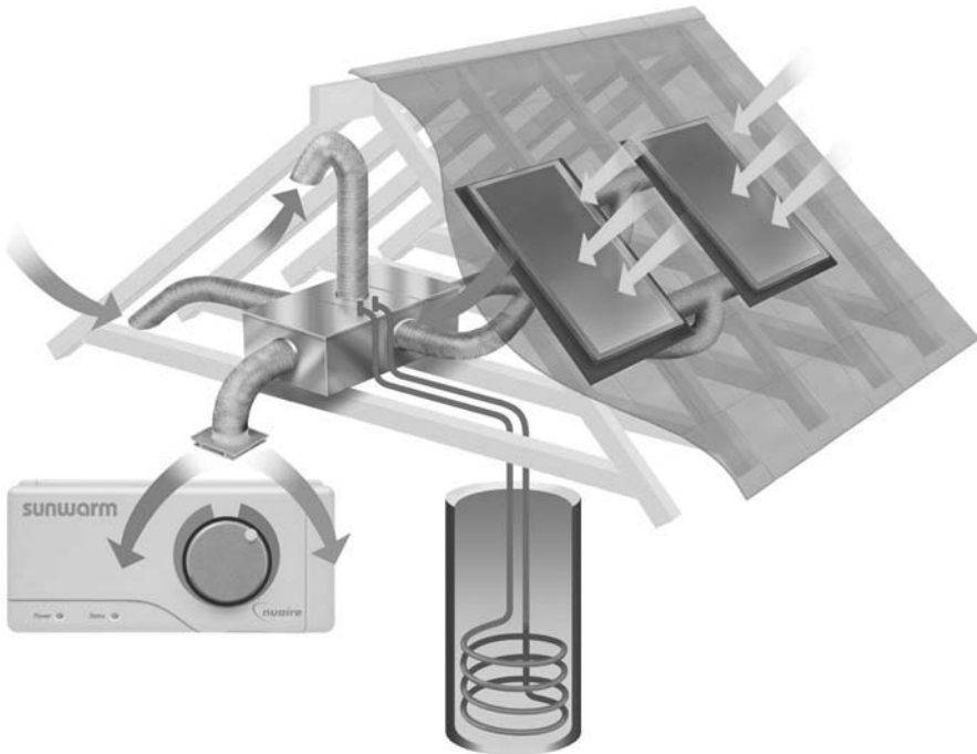
The Sunwarm warm air space heating system uses heat from TAPs and the attic, and can also provide DHW (Reproduced with permission from Nuaire)
