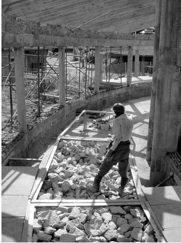
Rock bins using large aggregate have proved very effective (Reproduced with permission from Arup – Mike Rainbow)
