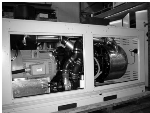
This Stirling engine generator set by STM Power produces 55kW and can run on biofuels and biogas (Reproduced with permission from Wtshymanski)
