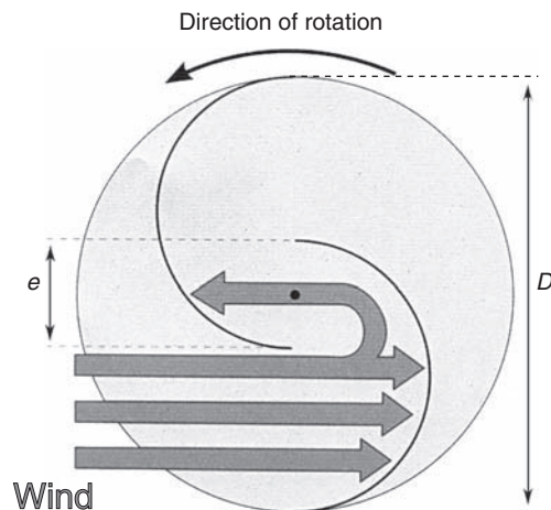
Principle of the Savonius turbine (Reproduced with permission from Schnargel)
