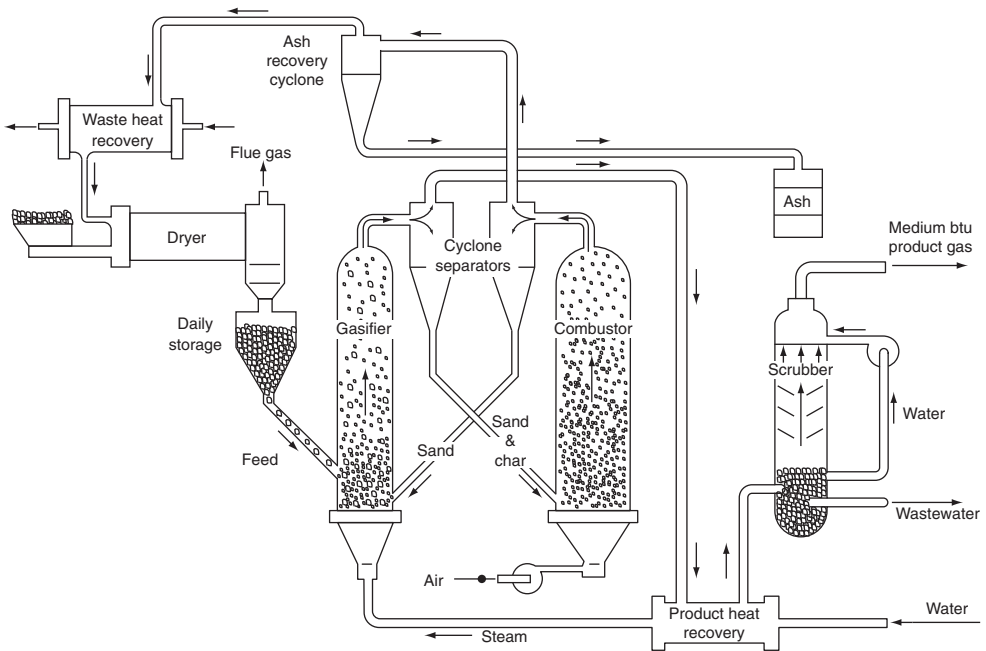
The Batelle process has a high throughput
