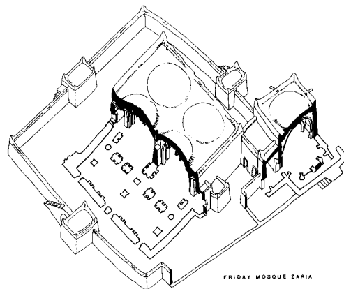
Figure 2.13 The Friday Mosque, Zaria: axonometric
