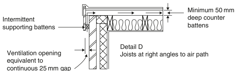
Figure 7.7 Roof ventilation less than 15^\circ
