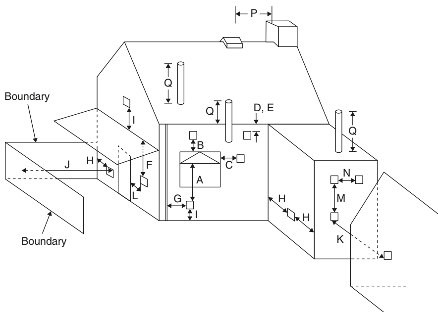
Figure 7.19 Locations of outlets from flues serving gas appliances (taken from Approved Document J). For labelling details, refer to Figure 7.20
