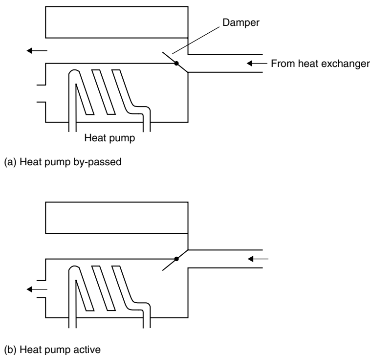
Figure 5.14 By-pass arrangement around heat pump
