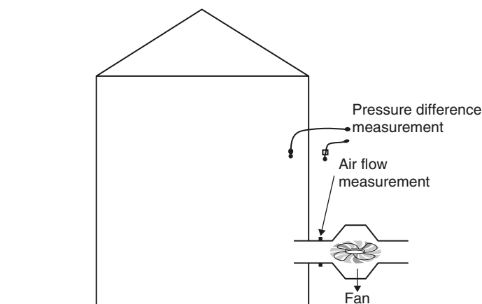
Figure 4.1 Fan-pressurisation testing schematic
