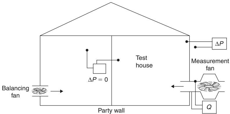
Figure 4.7 Pressure equalisation across party wall
